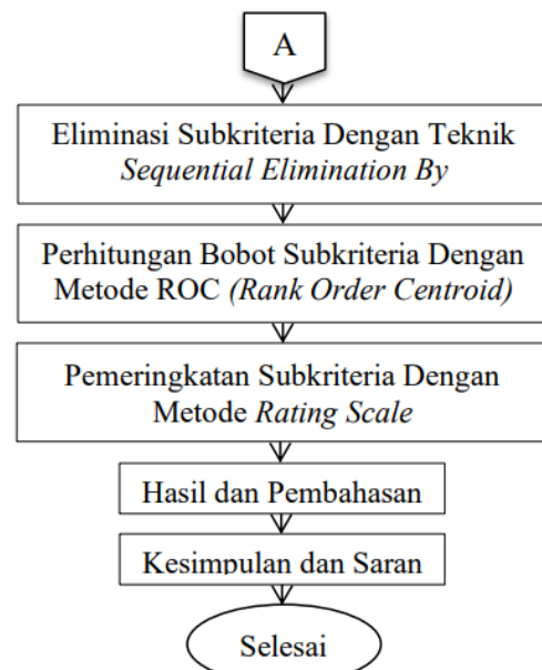
Gambar 1. Flowchart Penelitian
